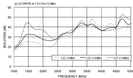
MCA-50LH ISOLATION L-R
