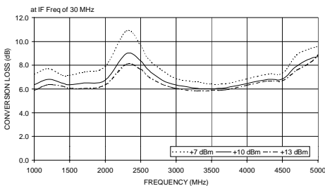
MCA-50LH CONVERSION LOSS
